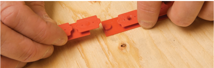
FIGURE 2.25: Snap together Nuheat Cable Guides
