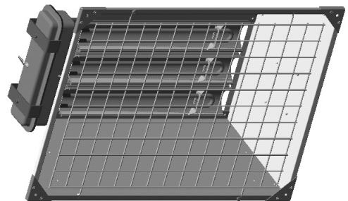
STAR-06 Fixed Heater After Grill has been Added See Page 3 – Fig. 2
