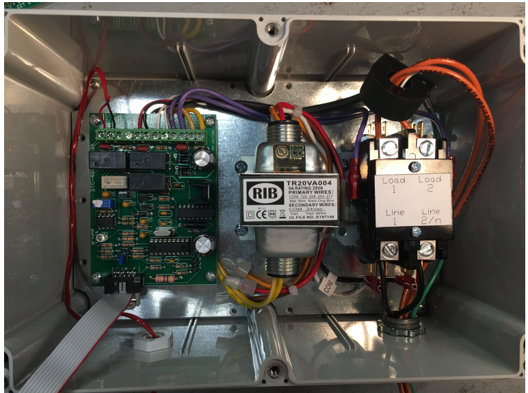
Does yours look like this? Note the load wires through the toroid coil (donut).
