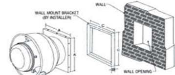
CDU Wall Mounting Details
