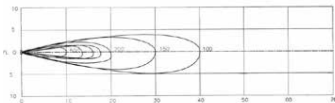
18" Horizontal Velocity Profile (Ft/Min)
