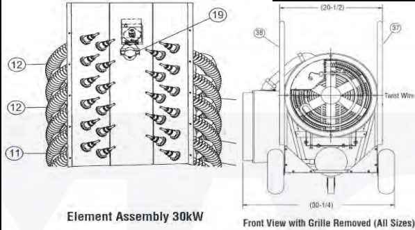
Front View with Grille Removed (All Sizes)
